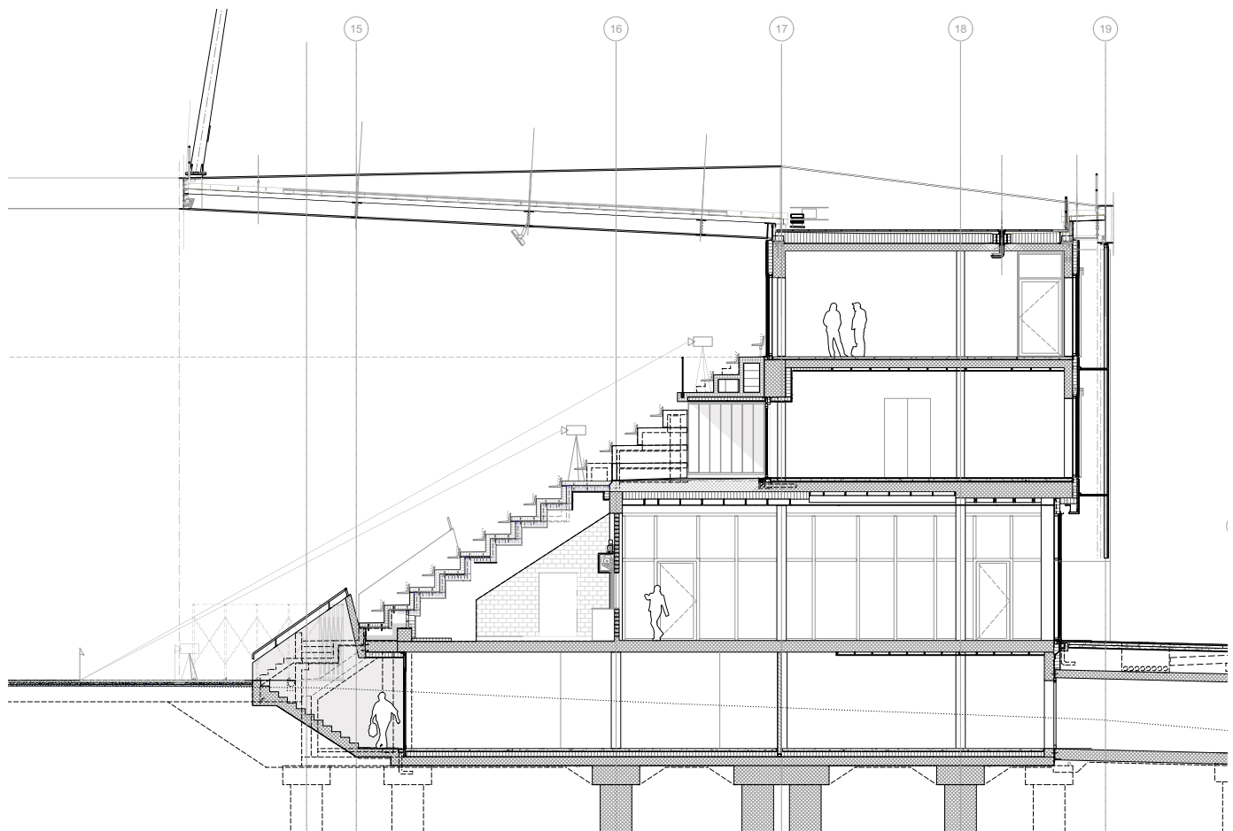
Coupe tribune principale
